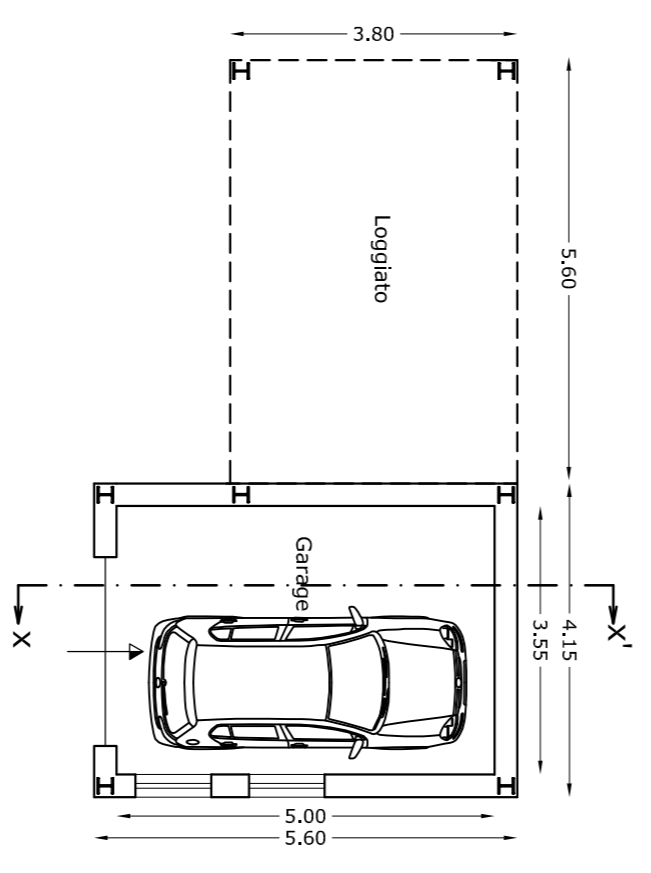
Piano Terra
